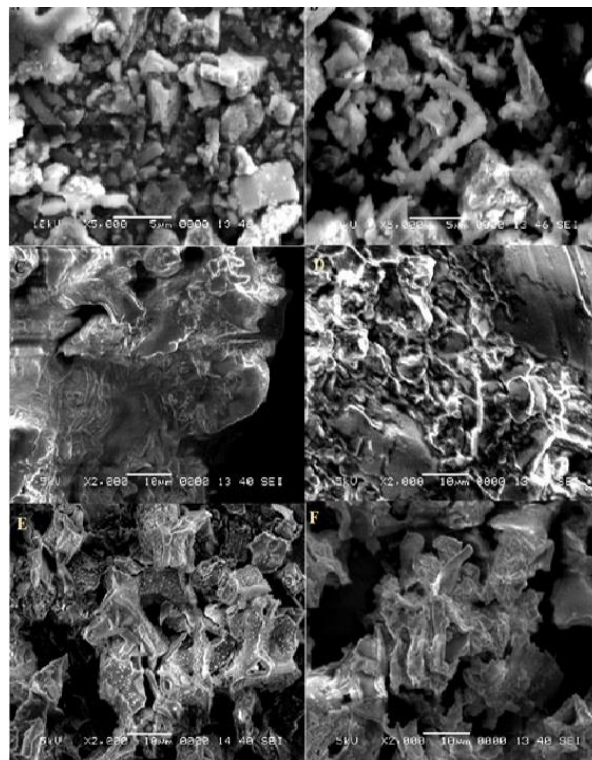
Figure 3: SEM results before and after removal study of indigo carmine on ESP, DPSP and PSP
