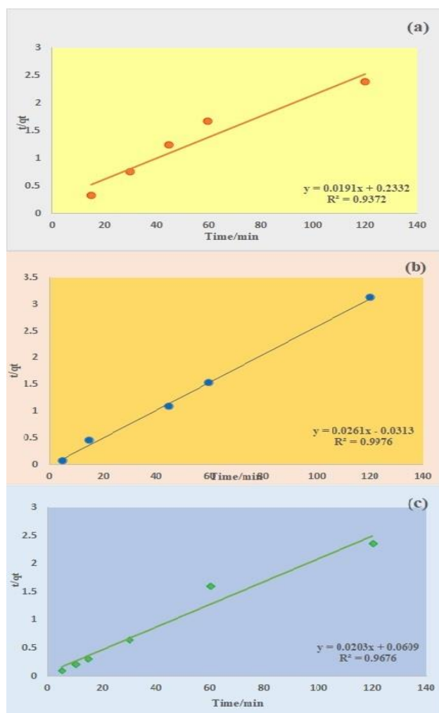
Figure 9: Kinetic pseudo second order model (a) ESP (b) DPSP (c) PSP on indigo carmine
