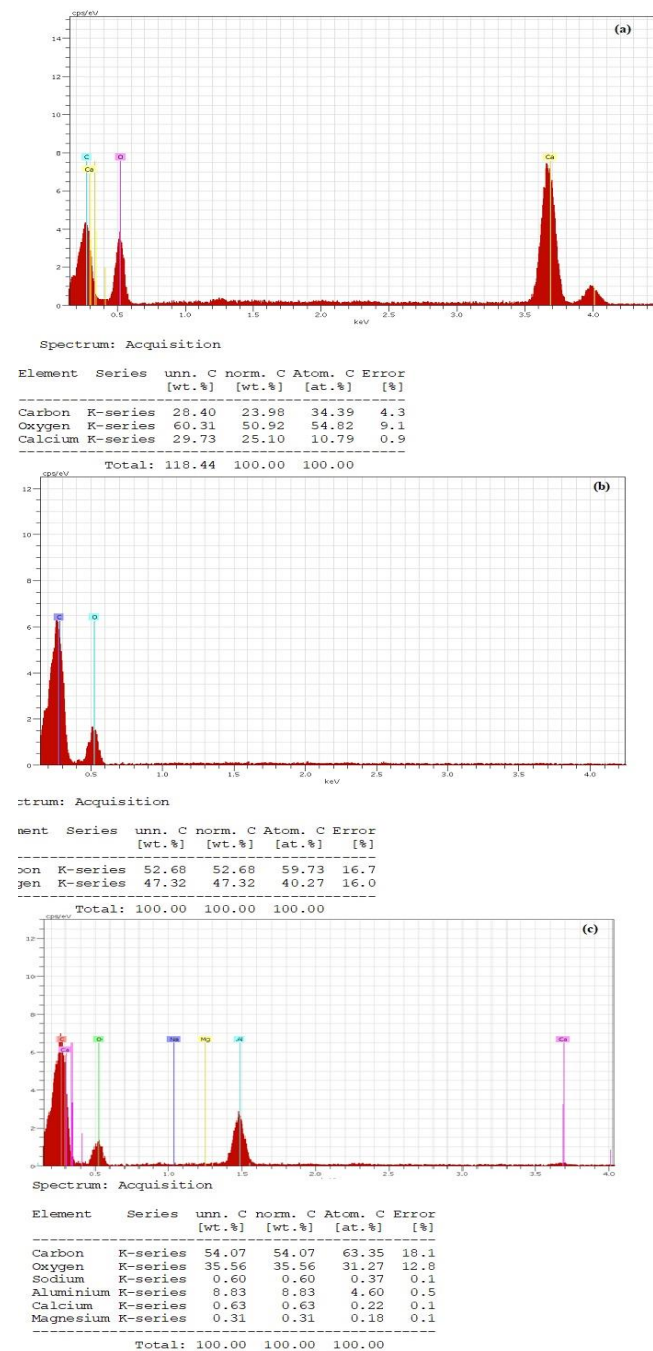
Figure 5: ESD Analysis of adsorbents before and after peaks A-ESP, B-DPSP and C-PSP
