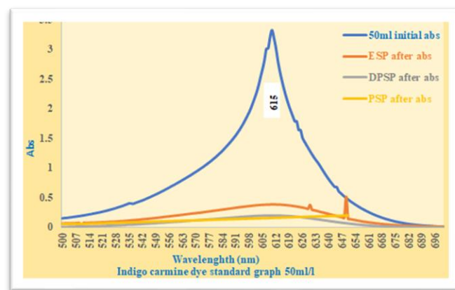
Figure 10: Standard graph shows initial and removal abs at 615(nm) indigo carmine dye
