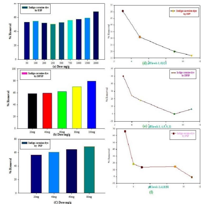
Figure 6: Effect of dose study of indigo carmine dye on adsorbents (a) ESP, (b) DPSP, (c) PSP while (d) ESP (e) DPSP (f) PSP Effect of pH study of Indigo carmine
